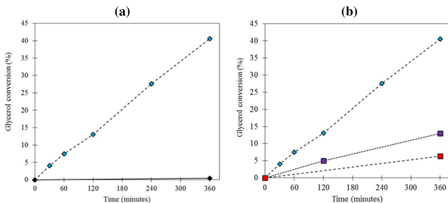
Fig. 3 a The effect of gas composition on glycerol conversion rates. Blue diamond 5% H_2 /CO 2 with 25% O_2 /CO 2 versus Black square 25% O_2 /CO 2 . b Glycerol conversion over 0.5 wt.% Pd/SiO 2 Violet square, 0.5 wt.% Fe/SiO 2 Red square and 0.5 wt.%Pd-0.5 wt.%Fe/SiO 2 Blue diamond catalysts with H_2O_2 generated in situ. Reaction Conditions: 10 g 0.3 M glycerol solution, 420 psi 5% H_2 / CO 2 , 160 psi 25% O_2 / CO 2 , 50 mg of catalyst, 1200 rpm stirring, 30 °C. (Color figure online)
